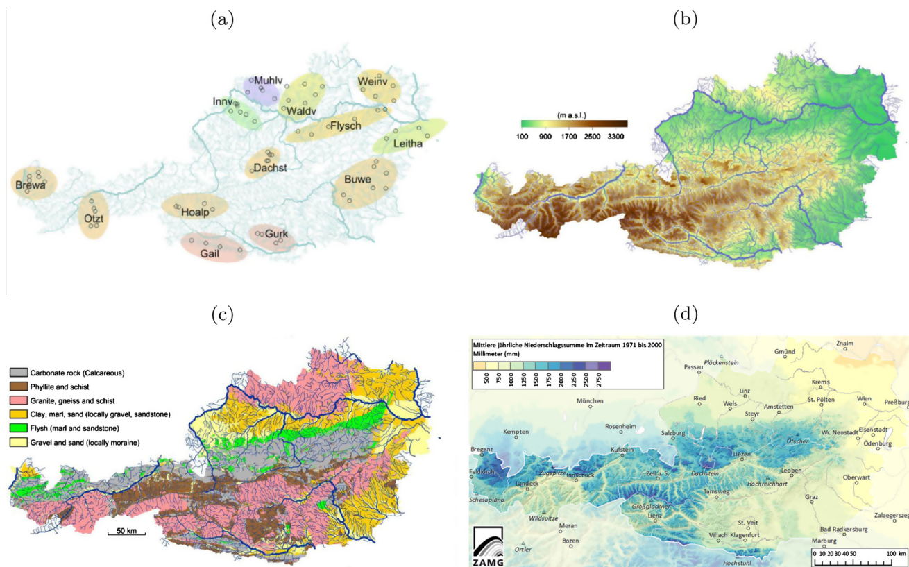
Fig. 1. Some characteristics of the study area: (a) clusters, (b) topography, (c) geology (all from Gaál et al. (2012), reprinted with permission from the publisher Wiley), and (d) mean annual precipitation (from ZAMG).
