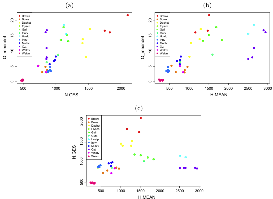
Fig. 5. Relation between the average deficit of droughts in discharge ( Q_{\text{meandef}} ) and (a) mean annual precipitation (N.GES), and (b) average elevation (H.MEAN), and (c) the relation between N.GES and H.MEAN; colour coded per cluster.
